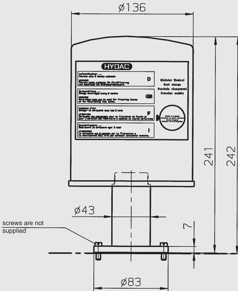
Flange model
