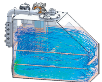
AFTER tank optimisation 550 litre tank volume
