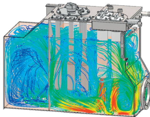
BEFORE tank optimisation 715 litre tank volume
