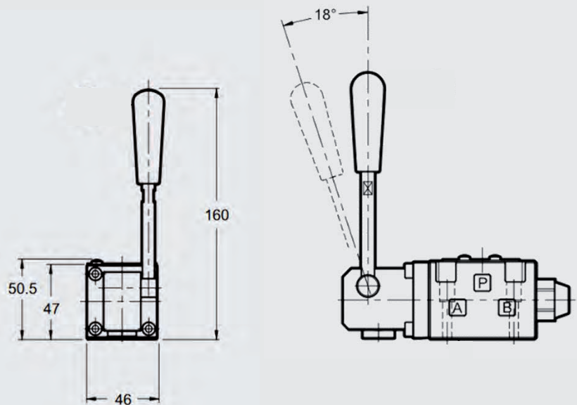
4/2-way
