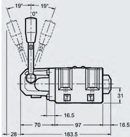
4/3-way
