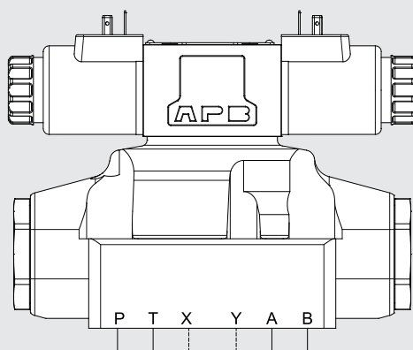
Directional valve
