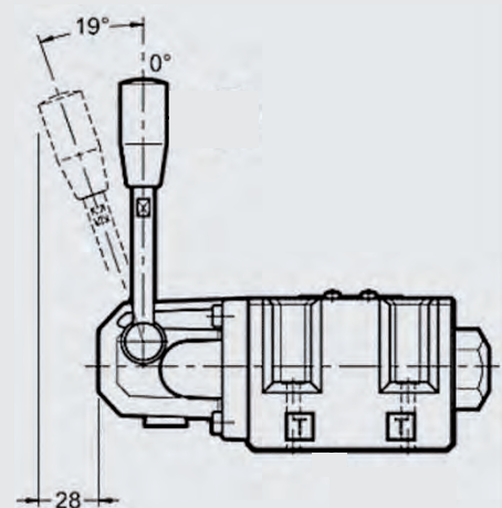
4/2-way
