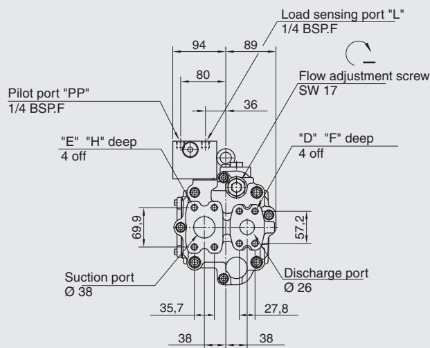
View X
