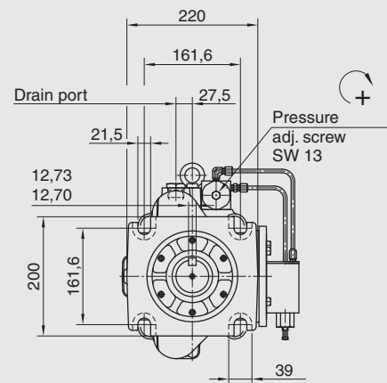
View X
