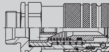
Push fit coupling ISO16028, flat face
