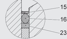
Detail "X" (2:1)
