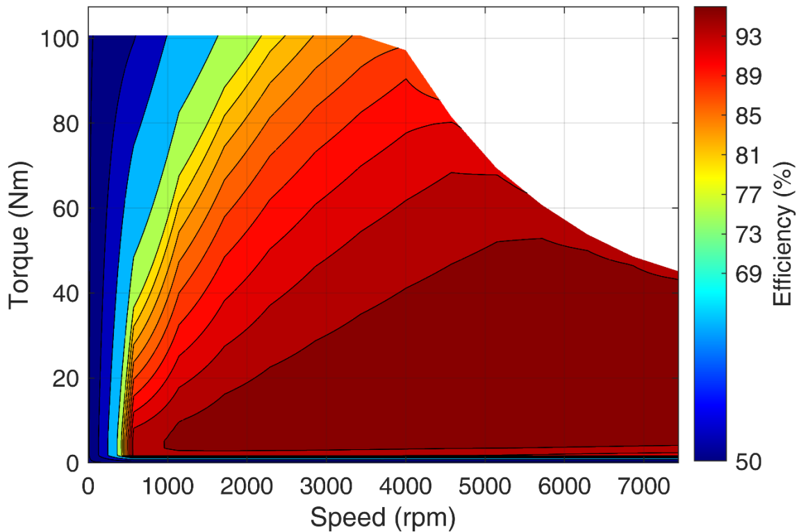
Simulated Efficiency of Motor Application (electric machine only; U_{nom} = 96 \text{ V} ; machine at 140^\circ \text{C} ;) )
